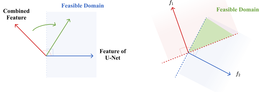
Figure 3: The left image shows the feature injection process in MIControlNet, while the right image illustrates the feature combination process. The Feasible Domain is where the combined optimization direction aligns with the U-Net feature or both control signal features f_1 and f_2 .
